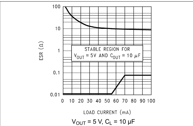
図 7-4. 5-V, 10- \mu\text{F} ESR Curves (Legacy Chip)
