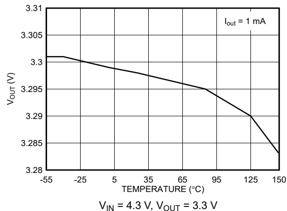
5-4. Output Voltage vs Temperature (New Chip)
