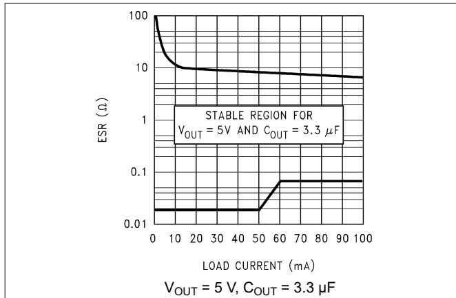
図 7-3. 5-V, 3.3- \mu\text{F} ESR Curves (Legacy Chip)
