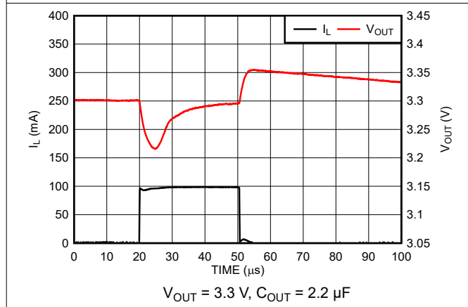
7-9. Load Transient Response (New Chip)
