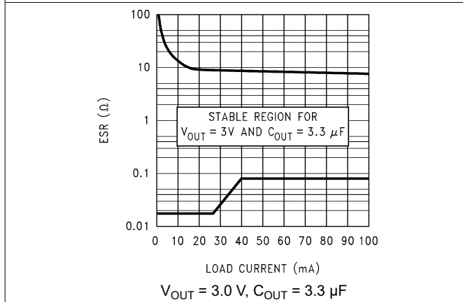
図 7-5. 3.0-V, 3.3- \mu\text{F} ESR Curves (Legacy Chip)
