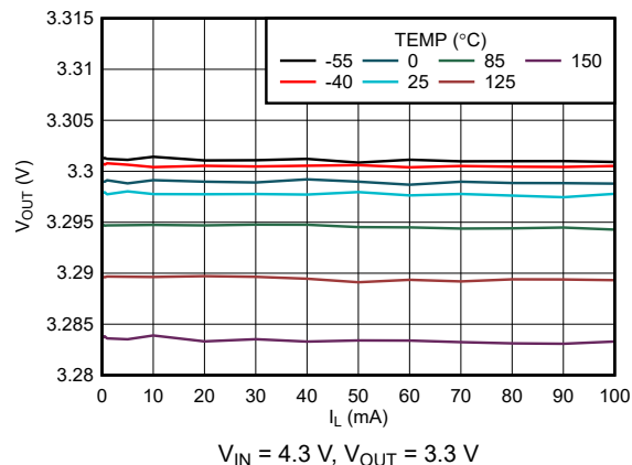
5-2. Output Voltage vs Load Current (New Chip)
