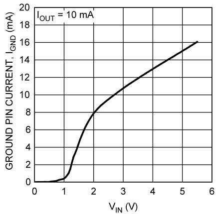
Ground Pin Current ( I_{GND} ) vs V_{IN}
