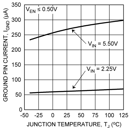
Ground Pin Current ( I_{GND} ) vs Temperature
