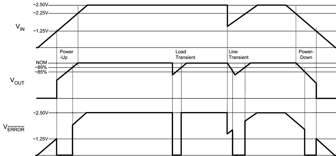
FIGURE 2. \overline{\text{ERROR}} Flag Operation, biased from V_{\text{IN}}
