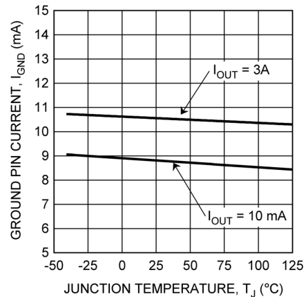
Ground Pin Current ( I_{GND} ) vs Temperature
