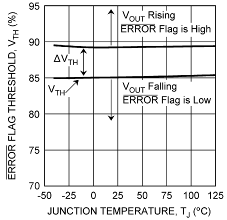
V_{OUT} ERROR Flag Threshold vs Temperature
