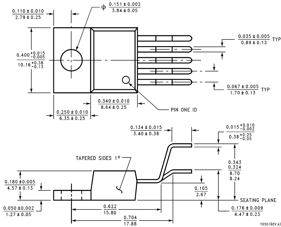
TO220 5-lead, Molded, Stagger Bend Package NS Package Number T05D
