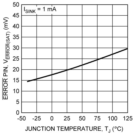
ERROR Flag Low vs Temperature
