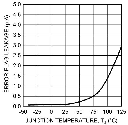
ERROR Flag Leakage vs Temperature
