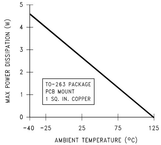
FIGURE 4. Maximum Power Dissipation vs Ambient Temperature for the TO-263 Package
