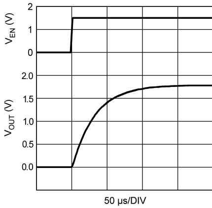
V_{OUT} vs V_{EN}
