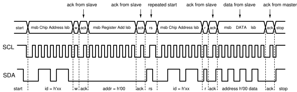
図 6-5. LP3943 Register Read
