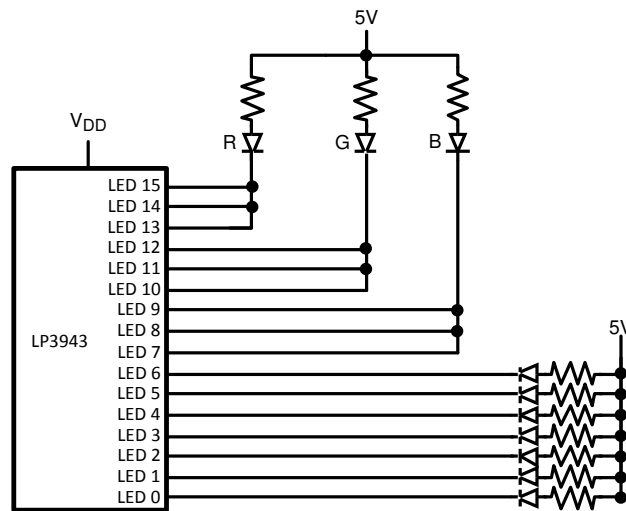
☒ 7-5. LP3943 Driving RGB LED as a Flash
