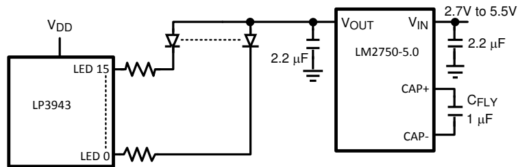
☒ 7-4. LP3943 With 5V Booster
