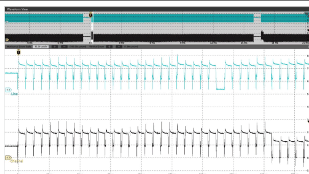
図 7-8. Line and Channel Waveform in One Frame (GSn = 0x0001h)
