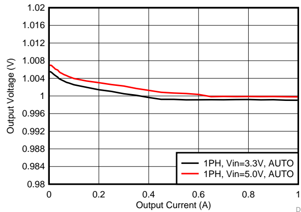
图 53. Output Voltage vs Load Current in PFM/PWM Mode (1-Phase Output)
