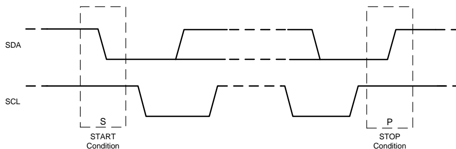
⊗ 23. Start and Stop Sequences
