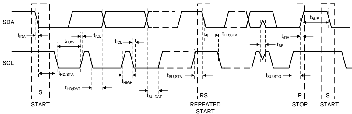
⊠ 1. I 2 C Timing
