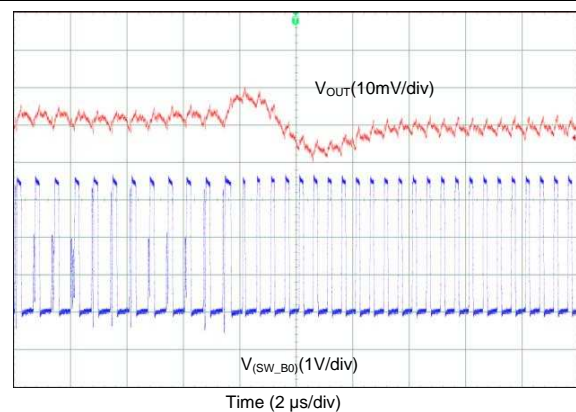
⊗ 87. Transient from PFM-to-PWM Mode (2-Phase Output)
