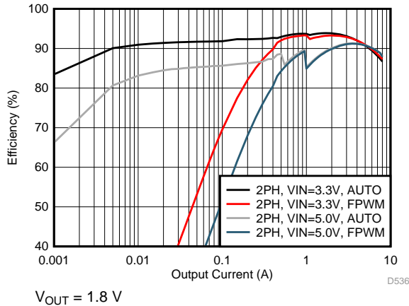
36. Efficiency in PFM/PWM and Forced-PWM Mode (2-Phase Output)
