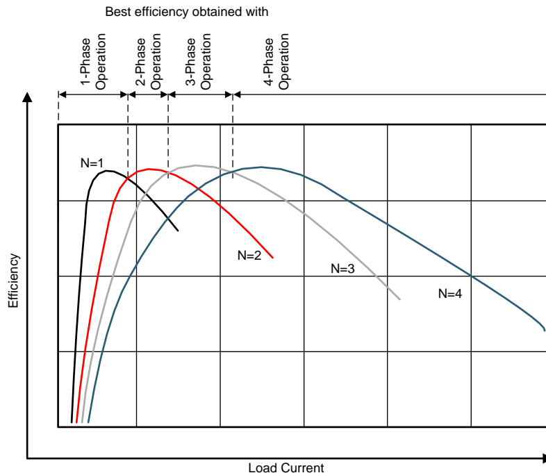
✎ 11. Multiphase Buck Converter Efficiency vs Number of Phases (Converters in PWM Mode)
