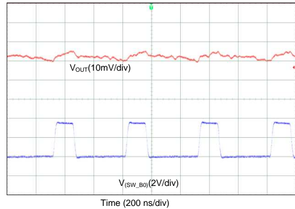
⊗ 83. Output Voltage Ripple, Forced-PWM Mode (2-Phase Output)
