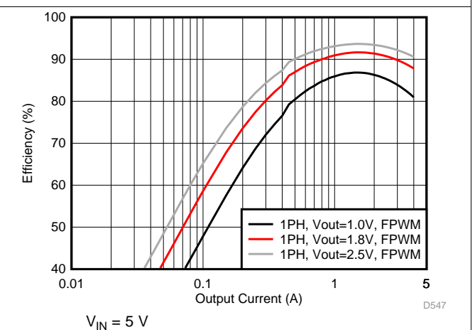
45. Efficiency in Forced-PWM Mode (1-Phase Output)
