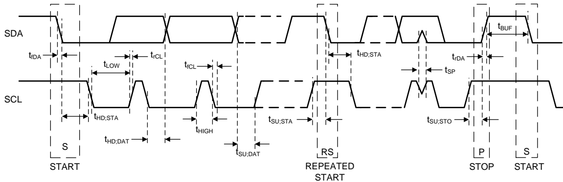
24. I 2 C-Compatible Timing
