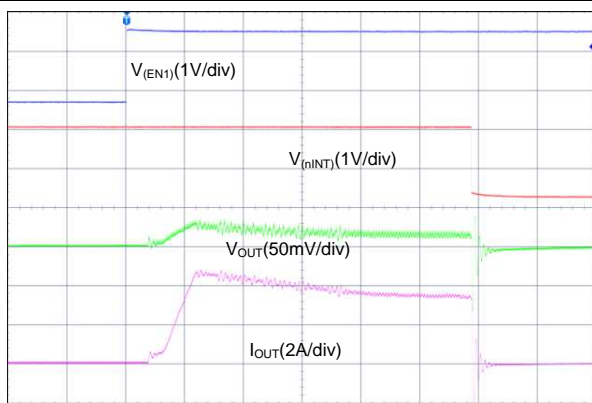
Time (200 \mu\text{s}/\text{div} )
