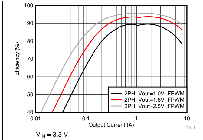
40. Efficiency in Forced-PWM Mode (2-Phase Output)
