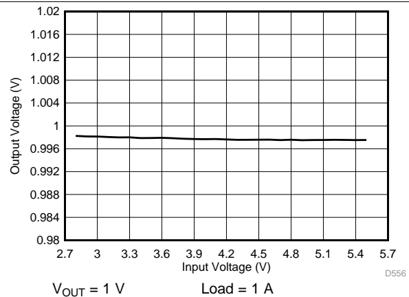
图 57. Output Voltage vs Input Voltage in PWM Mode (1-Phase Output)
