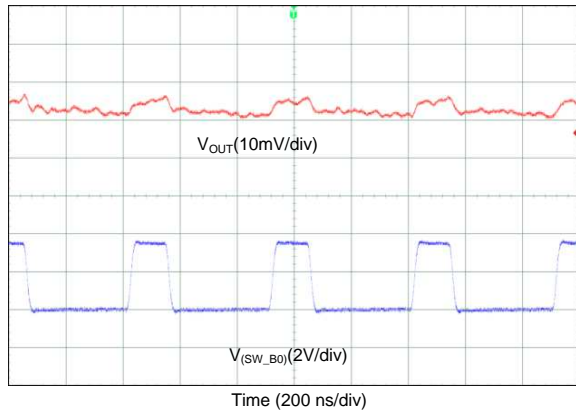
⊗ 82. Output Voltage Ripple, Forced-PWM Mode (3-Phase Output)
