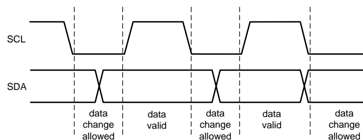
⊗ 22. Data Validity Diagram
