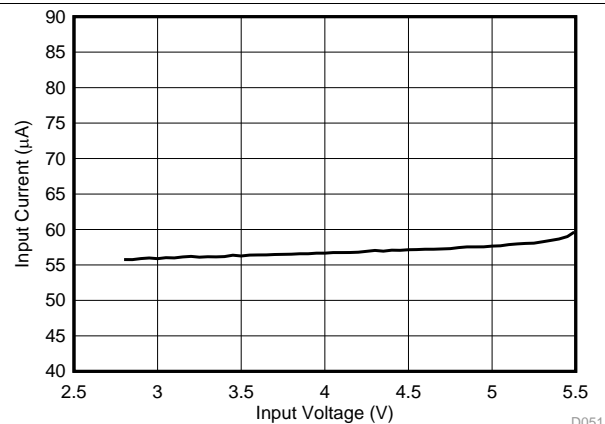
图 5. PFM Mode Current Consumption vs Input Voltage, One Regulator Enabled (3+1-Phase Output)
