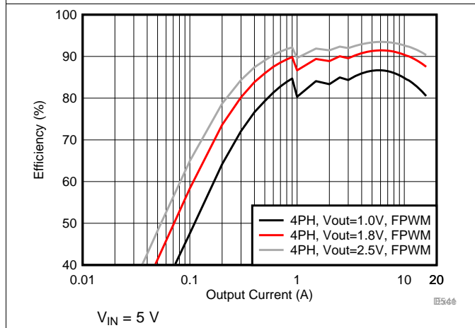
42. Efficiency in Forced-PWM Mode (4-Phase Output)
