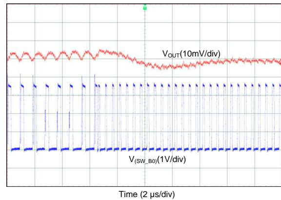
⊗ 85. Transient from PFM-to-PWM Mode (4-Phase Output)
