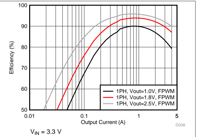
41. Efficiency in Forced-PWM Mode (1-Phase Output)
