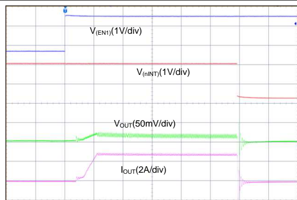
Time (200 \mu\text{s}/\text{div} )
