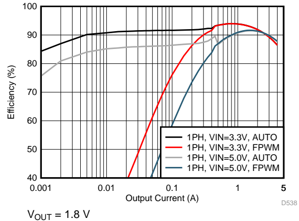
37. Efficiency in PFM/PWM and Forced-PWM Mode (1-Phase Output)
