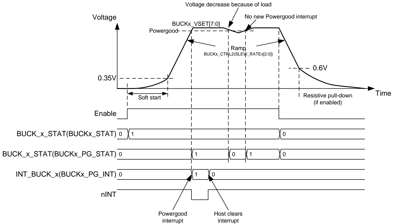
✎ 14. Regulator Enable and Disable
