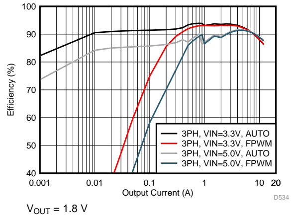
35. Efficiency in PFM/PWM and Forced-PWM Mode (3-Phase Output)
