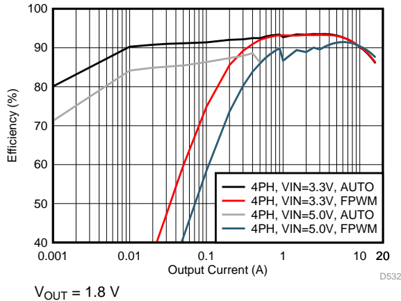
34. Efficiency in PFM/PWM and Forced-PWM Mode (4-Phase Output)
