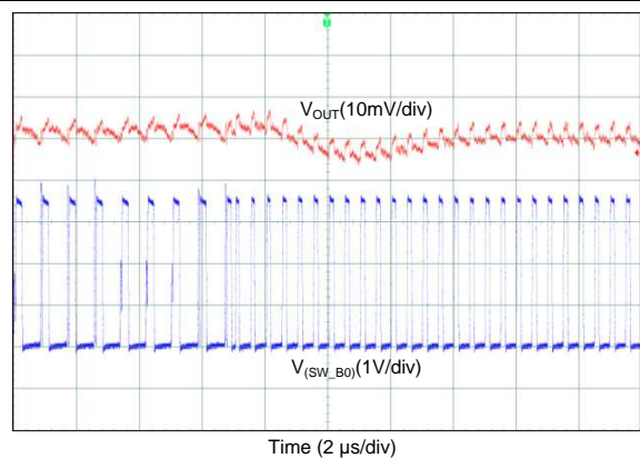
⊗ 84. Output Voltage Ripple, Forced-PWM Mode (1-Phase Output)
