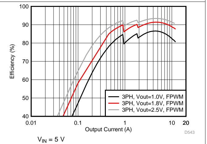
43. Efficiency in Forced-PWM Mode (3-Phase Output)
