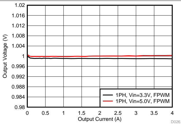
Fig 49. Output Voltage vs Load Current in Forced-PWM Mode (1-Phase Output)
