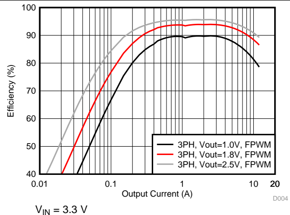
39. Efficiency in Forced-PWM Mode (3-Phase Output)
