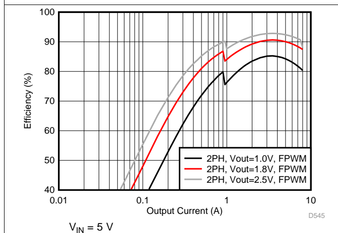
44. Efficiency in Forced-PWM Mode (2-Phase Output)
