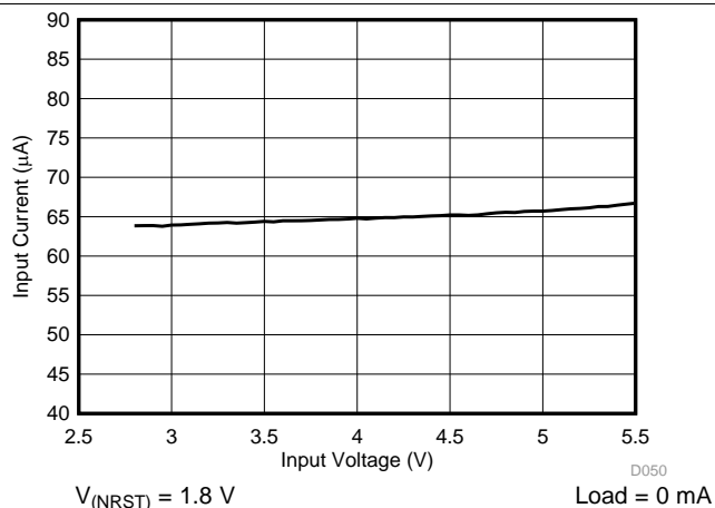
8. PFM Mode Current Consumption vs Input Voltage, One Regulator Enabled (2+2-Phase Output)
