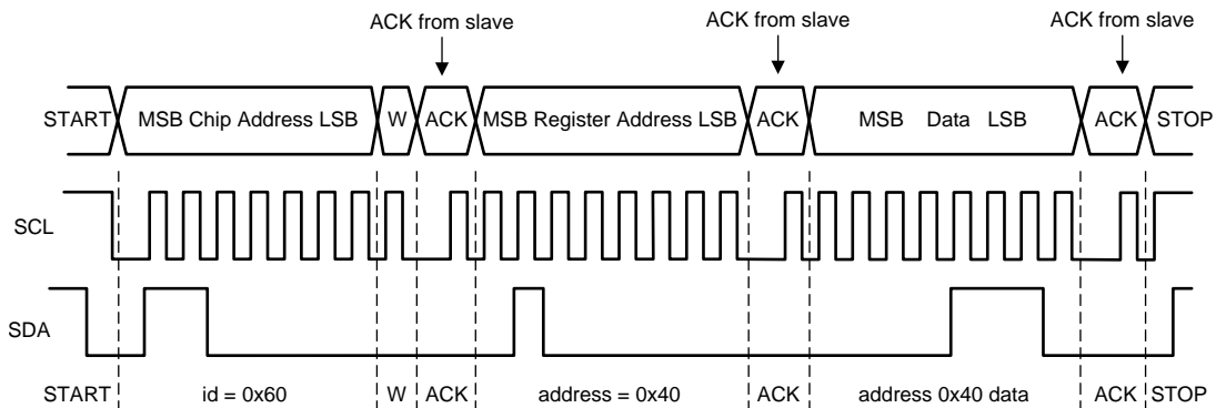
25. Write Cycle (w = write; SDA = 0), Using Example id = Device Address = 0x60 for LP8756x-Q1
