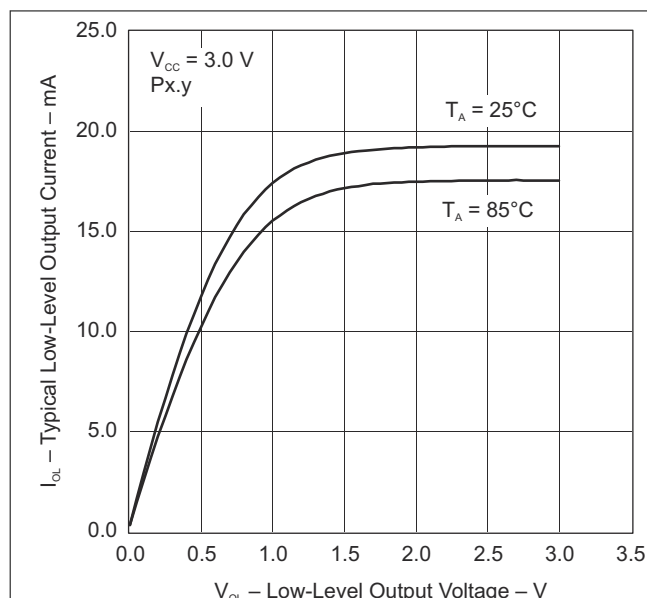
7-3. Typical Low-Level Output Current vs Low-Level Output Voltage
