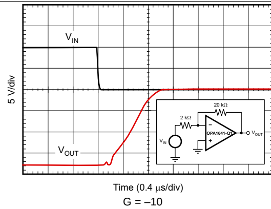
Figure 18. Negative Overload Recovery
