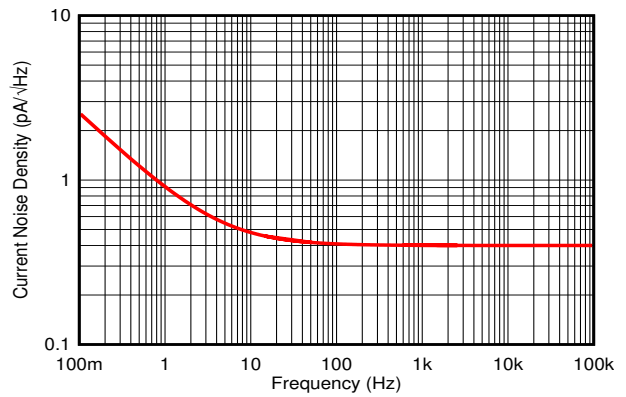
6-4. Input Current Noise Spectral Density vs Frequency
