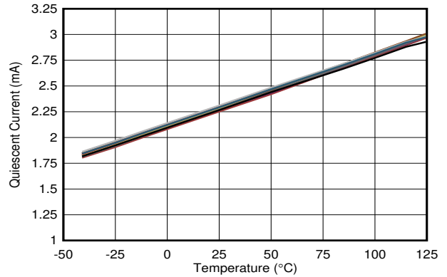
6-26. Quiescent Current vs Temperature
