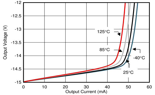
6-28. Output Voltage vs Output Current (Sinking)
