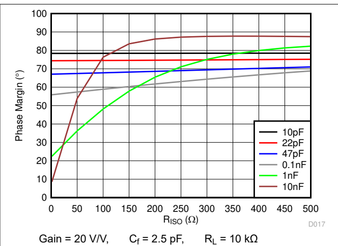
図 8-3. Phase Margin vs. Series Isolation Resistor
