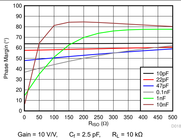
図 8-2. Phase Margin vs. Series Isolation Resistor
