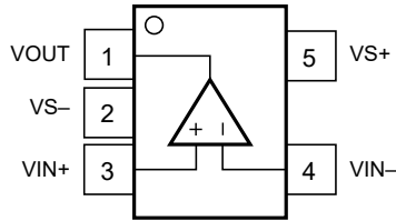
図 5-1. OPA863A DBV Package, 5-Pin SOT-23 (Top View)
