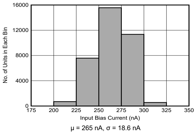
6-17. Input Bias Current Distribution
