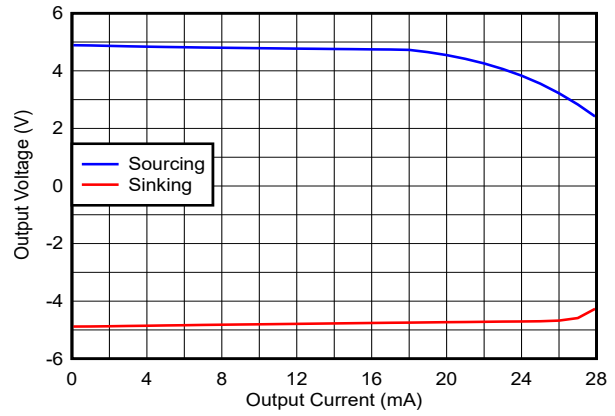
6-14. Output Voltage vs Load Current
