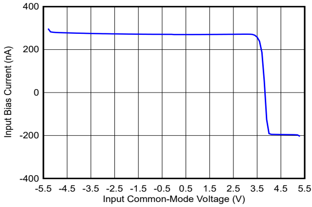
6-13. Input Bias Current vs Input Common-Mode Voltage
