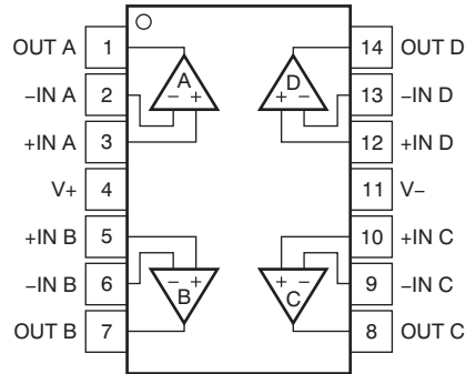
Pin Functions: OPA4322-Q1
