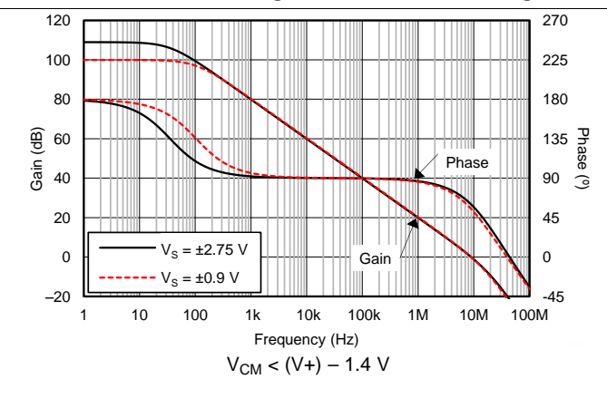
Fig 6. Open-Loop Gain and Phase vs Frequency
