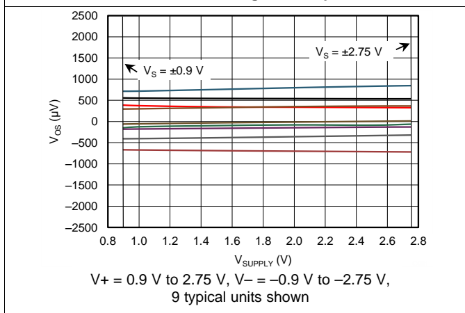
Fig 5. Offset Voltage vs Power Supply
