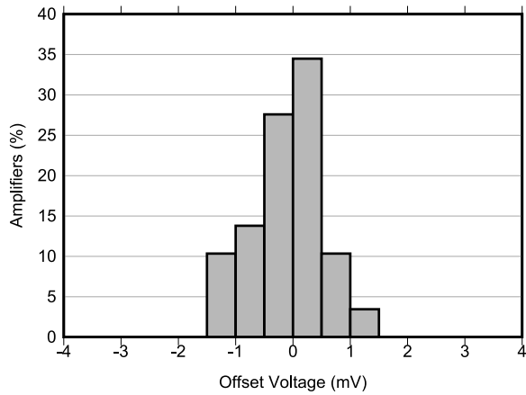
6-1. Offset Voltage Distribution at 25°C
