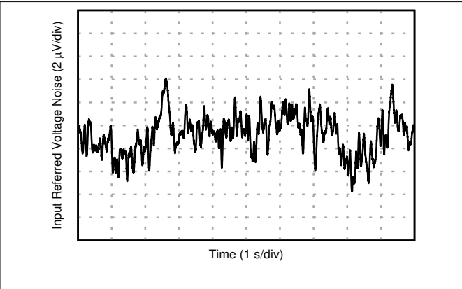
6-50. 0.1-Hz to 10-Hz Noise
