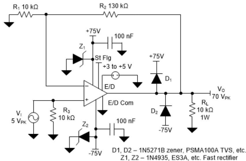
図 8-1. OPA455, High-Voltage Noninverting Amplifier, A_V = 14 V/V
