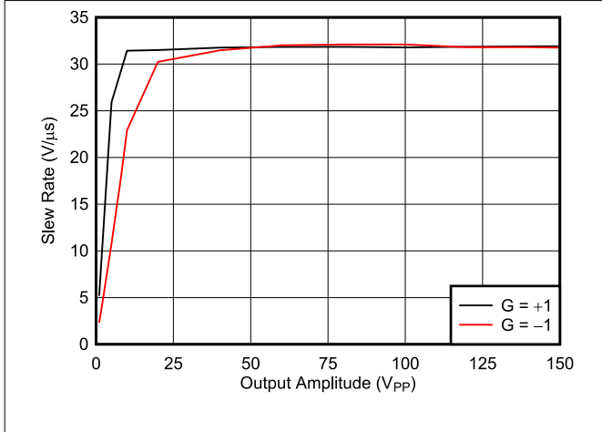
Figure 6-43. Slew Rate vs Output Step Size
