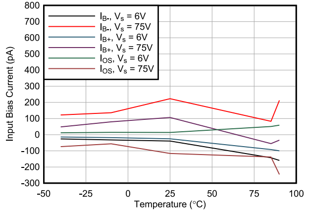
6-20. IB vs Temperature
