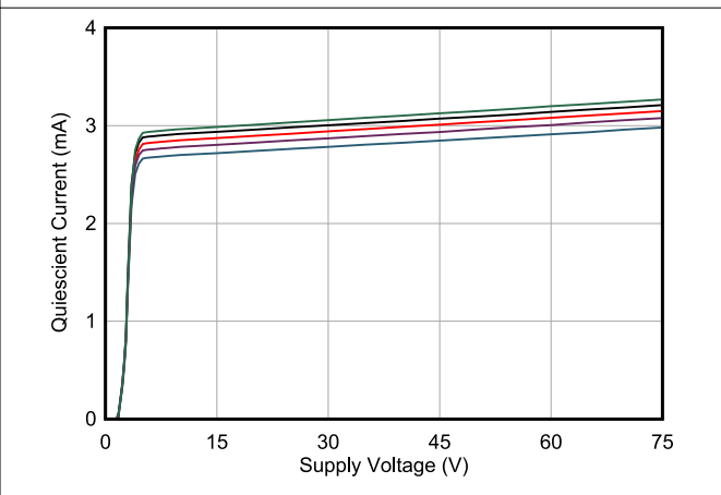
6-54. Quiescent Current vs Supply Voltage
