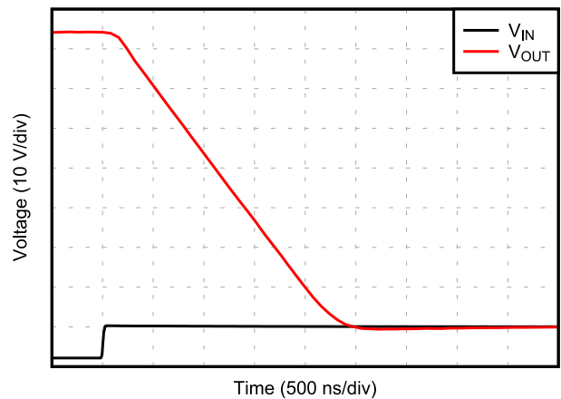
6-34. Positive Overload Recovery
