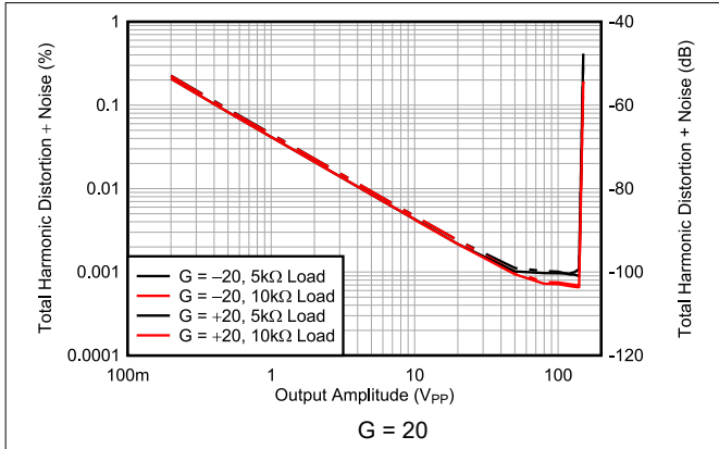
6-49. THD+N Ratio vs Output Amplitude
