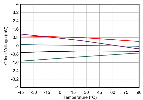
6-5. Offset Voltage vs Temperature
