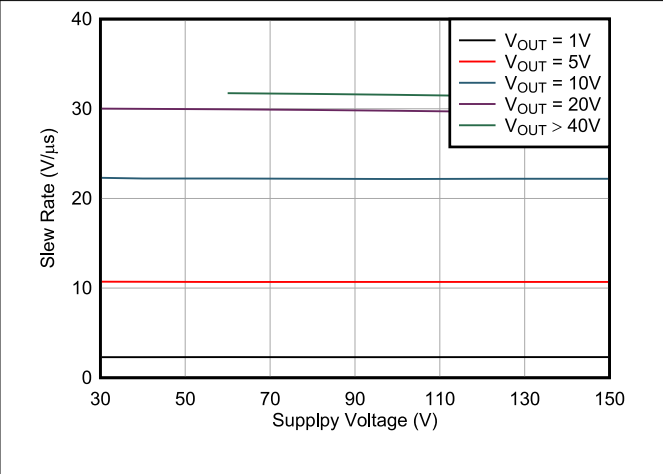
Figure 6-44. Slew Rate vs Supply Voltage (Inverting)
