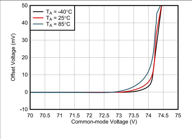
6-8. Offset Voltage vs Common-Mode Voltage (High V_{CM} )
