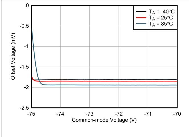
6-7. Offset Voltage vs Common-Mode Voltage (Low V_{CM} )
