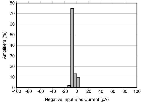
6-19. Input Bias Current Production Distribution at 25°C
