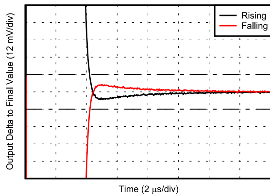
6-33. Negative Overload Recovery
