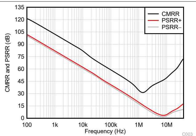
图 5-16. CMRR and PSRR vs Frequency
