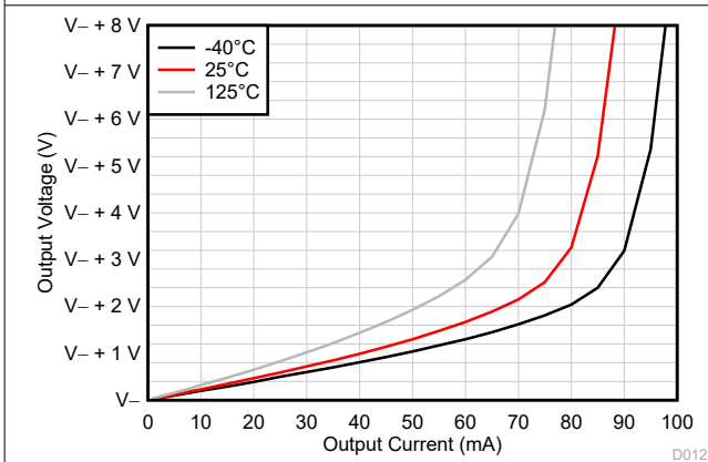
图 5-15. Output Voltage Swing vs Output Current (Sinking)
