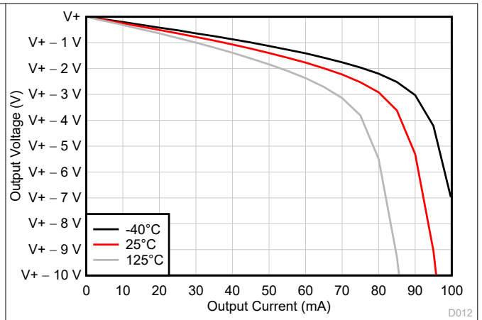
图 5-14. Output Voltage Swing vs Output Current (Sourcing)
