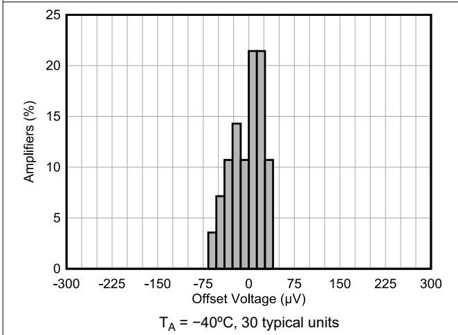
6-3. Input Offset Production Distribution
