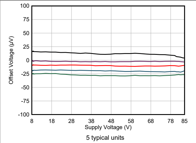
6-8. Input Offset Voltage vs Supply Voltage
