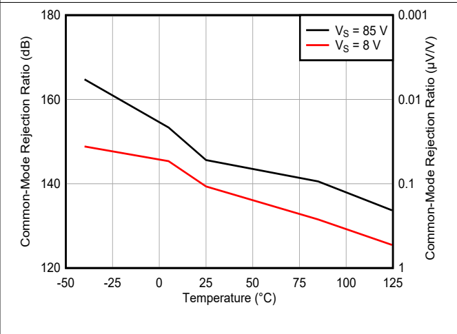
6-10. CMRR vs Temperature
