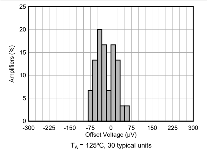
6-4. Input Offset Production Distribution
