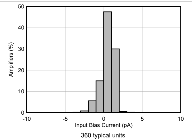
6-6. Input Bias Current Production Distribution
