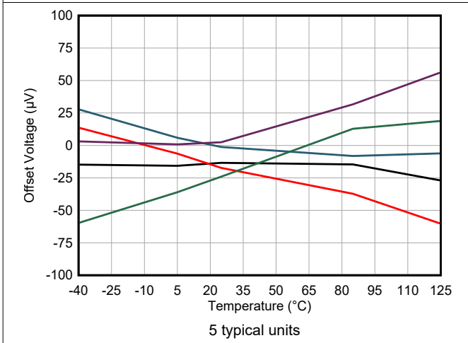
6-9. Input Offset Voltage vs Temperature
