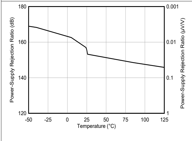
6-11. PSRR vs Temperature
