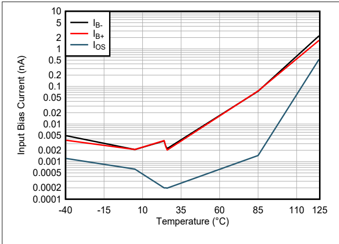
6-13. Input Bias Current and Current Offset vs Temperature
