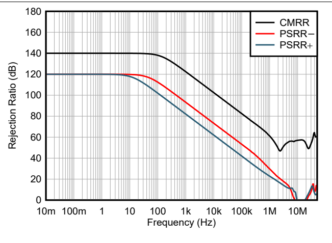
6-14. PSRR and CMRR vs Frequency
