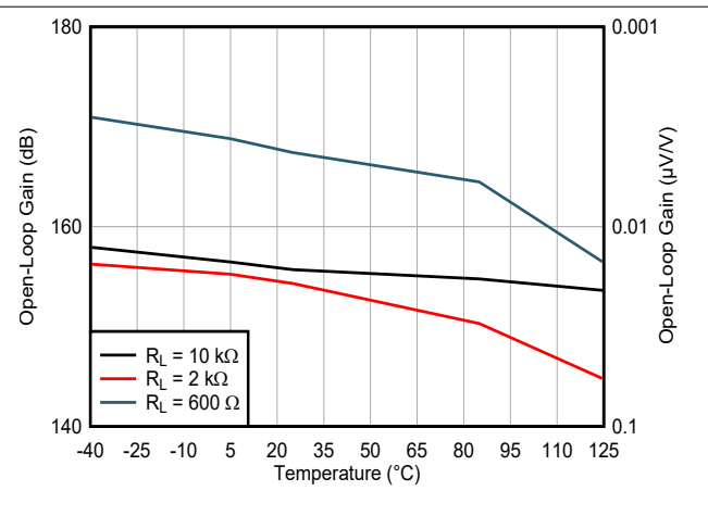
6-16. Open Loop Gain vs Temperature
