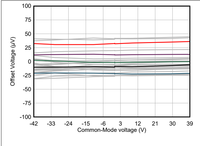
6-7. Input Offset Voltage vs Common-Mode Voltage
