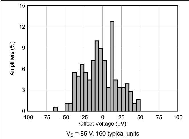
6-1. Input Offset Production Distribution
