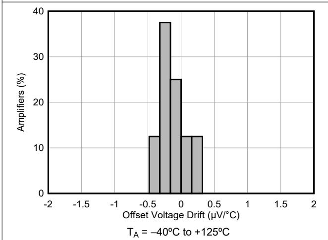
6-5. Input Offset Voltage Drift Distribution
