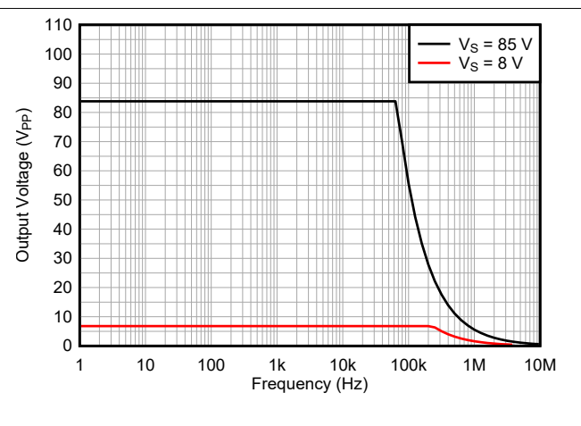
6-18. Maximum Output Voltage vs Frequency
