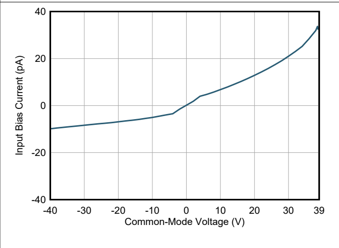
6-12. Input Bias Current vs Common-Mode Voltage
