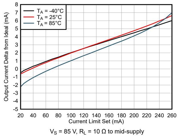
6-38. Output Sinking Current Error vs Current Limit Set
