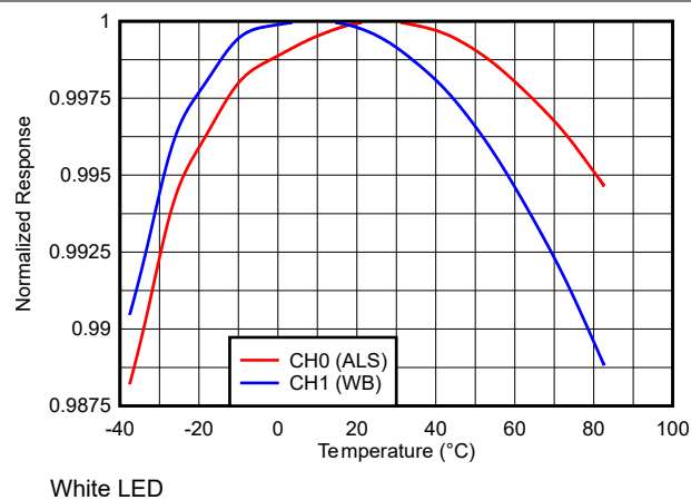
図 5-12. Device Response vs Temperature
