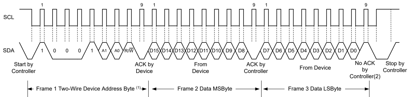
8-5. I 2 C Read Example
