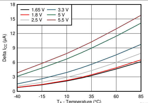
FIG 6-18. \Delta I_{CC} vs Temperature for Different V_{CC} ( V_I = V_{CC} - 0.6\text{ V} )
