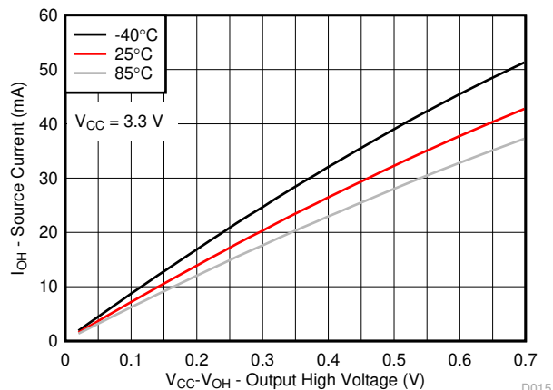
FIG 6-14. I/O Source Current vs Output High Voltage for Different Temperature ( T_A ) for V_{CC} = 3.3\text{ V}
