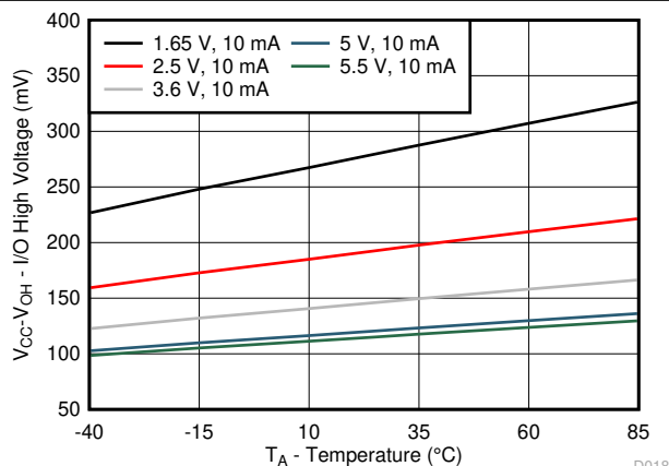
FIG 6-17. V_{CC} - V_{OH} Voltage vs Temperature for Different V_{CC}
