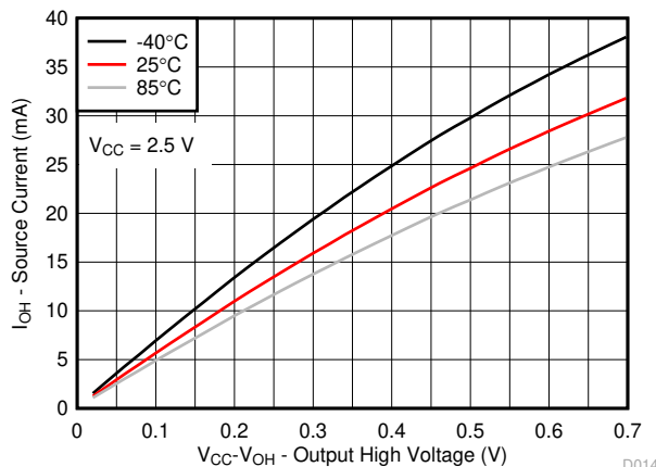
FIG 6-13. I/O Source Current vs Output High Voltage for Different Temperature ( T_A ) for V_{CC} = 2.5\text{ V}
