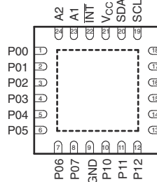
RTW PACKAGE (TOP VIEW)
