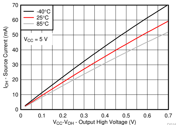
FIG 6-15. I/O Source Current vs Output High Voltage for Different Temperature ( T_A ) for V_{CC} = 5\text{ V}
