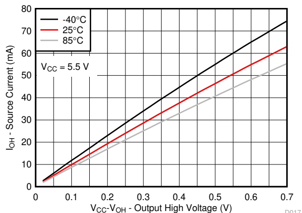
FIG 6-16. I/O Source Current vs Output High Voltage for Different Temperature ( T_A ) for V_{CC} = 5.5\text{ V}
