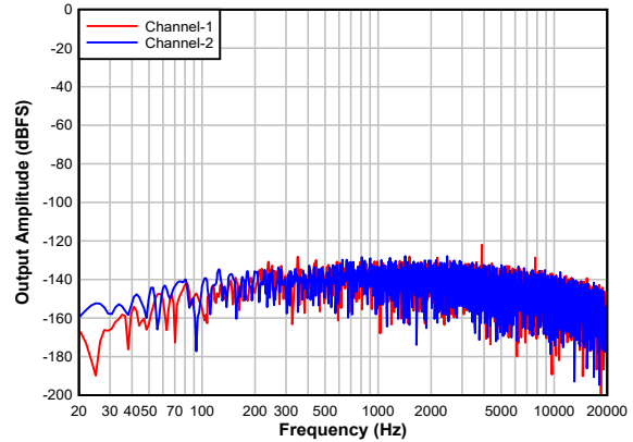
7-23. Single Ended FFT With Idle Input With DRE Disabled
