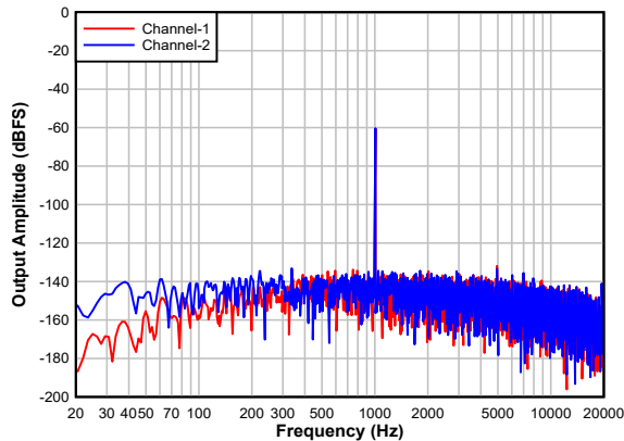
7-24. Single Ended FFT With a -60-dBr Input With DRE Enabled
