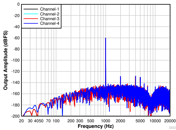
7-30. PDM Input FFT With a -60-dBr Input
