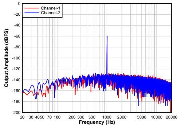
7-25. Single Ended FFT With a -60-dBr Input With DRE Disabled
