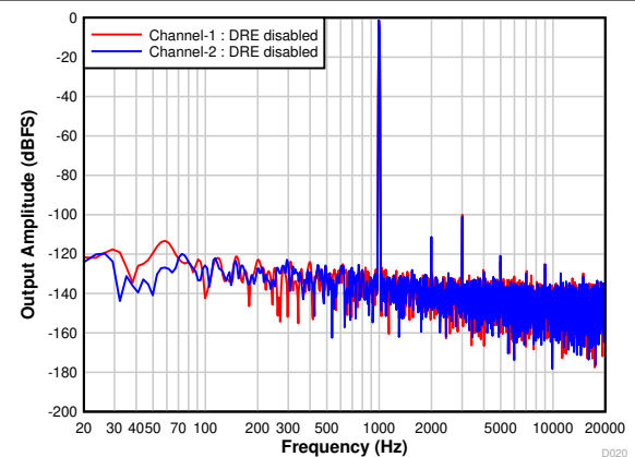
7-27. Differential FFT With a -1-dBr Input With DRE Disabled
