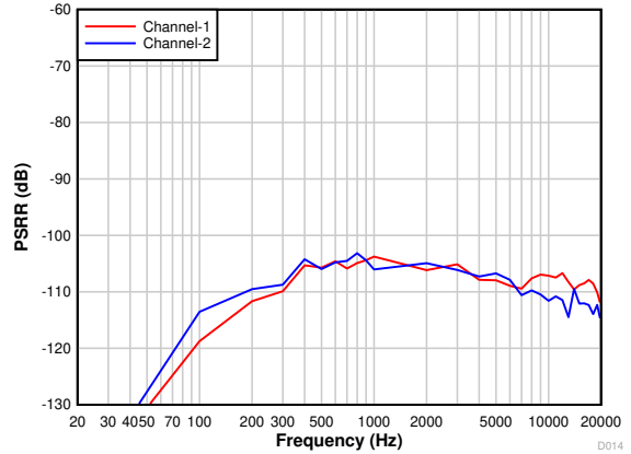
7-17. Power-Supply Rejection Ratio vs Ripple Frequency With 100-mV pp Amplitude
