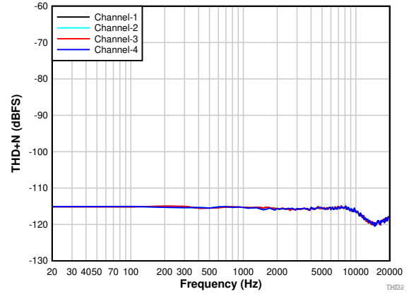
7-29. PDM Input THD+N vs Input Frequency With a -20-dBr Input
