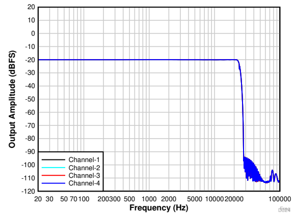
7-31. PDM Input Frequency Response With a -20-dBr Input
