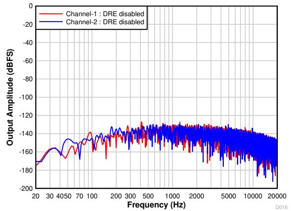
7-19. Differential FFT With Idle Input With DRE Disabled
