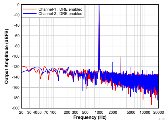
7-26. Differential FFT With a -1-dBr Input With DRE Enabled
