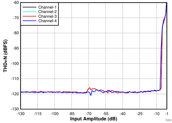
7-28. PDM Input THD+N vs Input Amplitude
