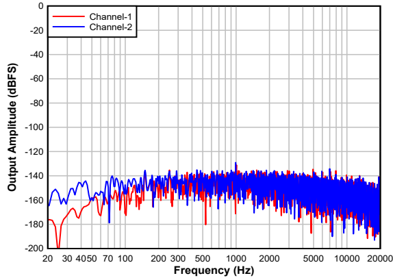
7-22. Single Ended FFT With Idle Input With DRE Enabled
