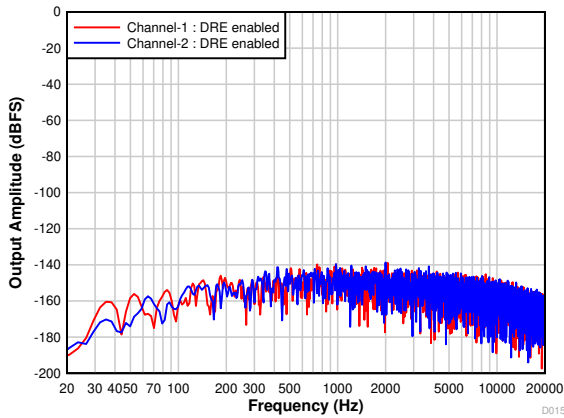
7-18. Differential FFT With Idle Input With DRE Enabled
