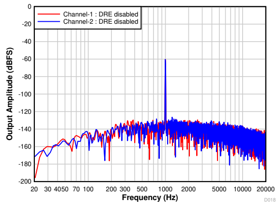
7-21. Differential FFT With a -60-dBr Input With DRE Disabled
