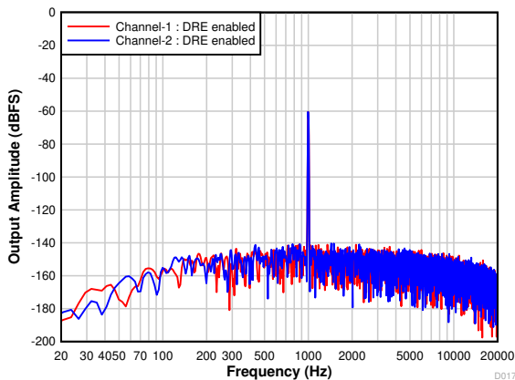
7-20. Differential FFT With a -60-dBr Input With DRE Enabled
