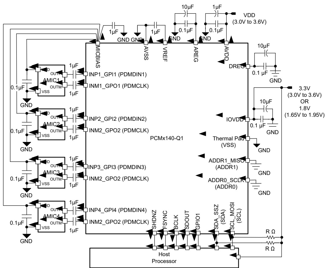
8-1. Four-Channel Analog Microphone Recording Diagram
