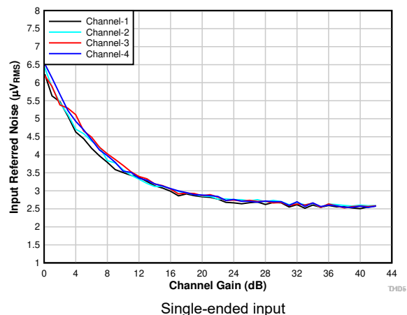
6-14. Input-Referred Noise vs Channel Gain
