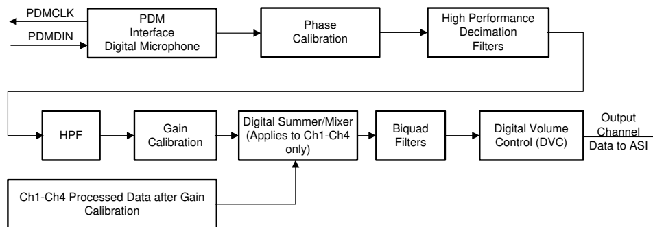
Figure 7-16. Signal-Chain Processing Flowchart
