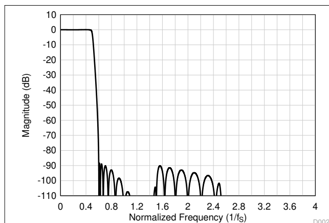
Figure 7-41. Low-Latency Decimation Filter Magnitude Response
