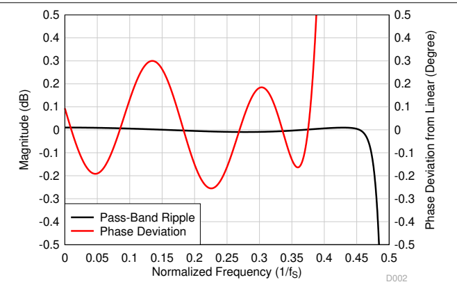
Figure 7-40. Low-Latency Decimation Filter Pass-Band Ripple and Phase Deviation
