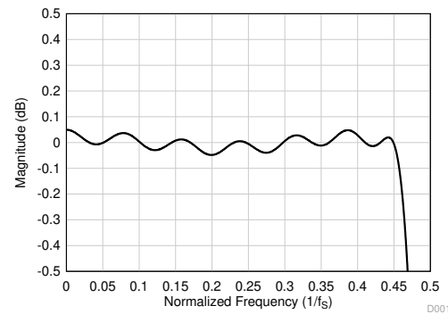
☒ 7-30. Linear Phase Decimation Filter Pass-Band Ripple
