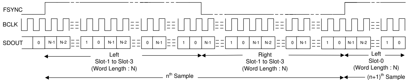
图 7-11. LJ Protocol Timing (No Idle BCLK Cycles, TX_OFFSET = 0)
