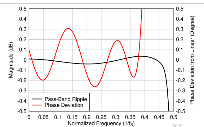
Figure 7-42. Low-Latency Decimation Filter Pass-Band Ripple and Phase Deviation
