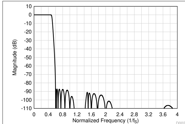
Figure 7-39. Low-Latency Decimation Filter Magnitude Response
