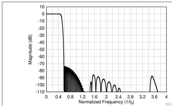
☒ 7-29. Linear Phase Decimation Filter Magnitude Response
