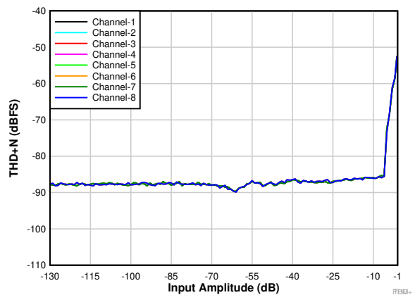
Fourth order PDM modulator with PDMCLKx = 1.536 MHz
