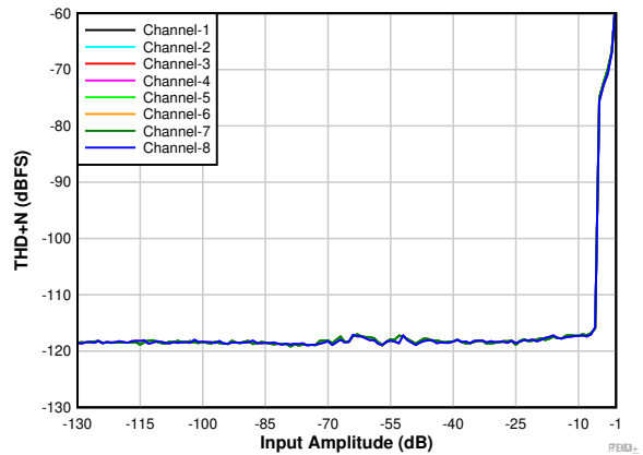
Fourth order PDM modulator with PDMCLKx = 3.072 MHz
