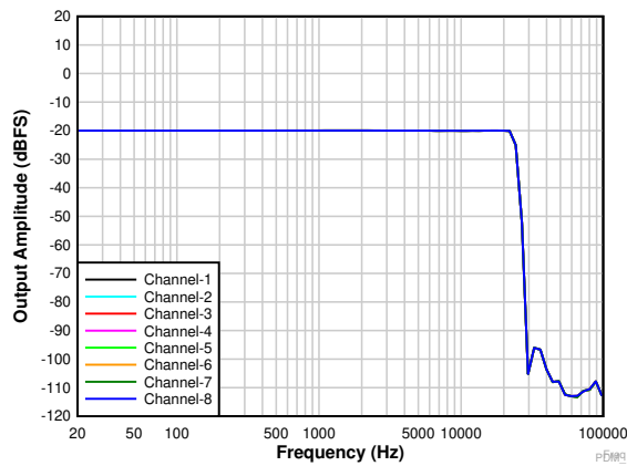
Fourth order PDM modulator with PDMCLKx = 3.072 MHz
