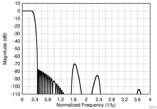
图 6-31. Linear Phase Decimation Filter Magnitude Response
