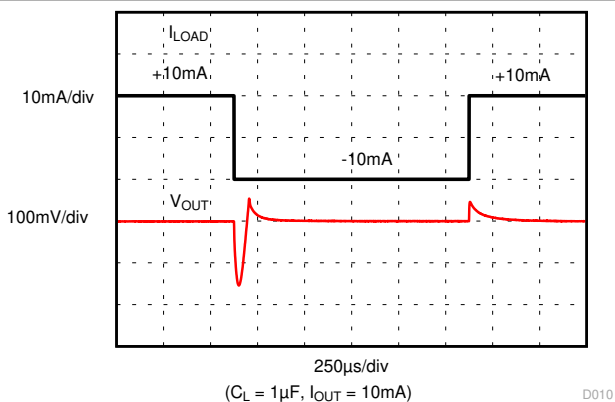
Figure 6-12. Load Transient
