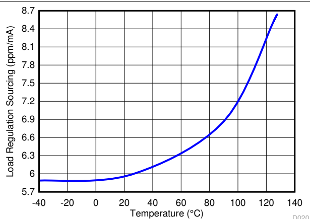
Figure 6-7. Load Regulation Sourcing
