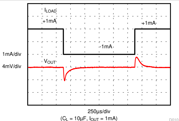
Figure 6-11. Load Transient
