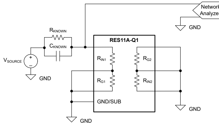
图 6-5. Capacitance Measurement Reference Schematic
