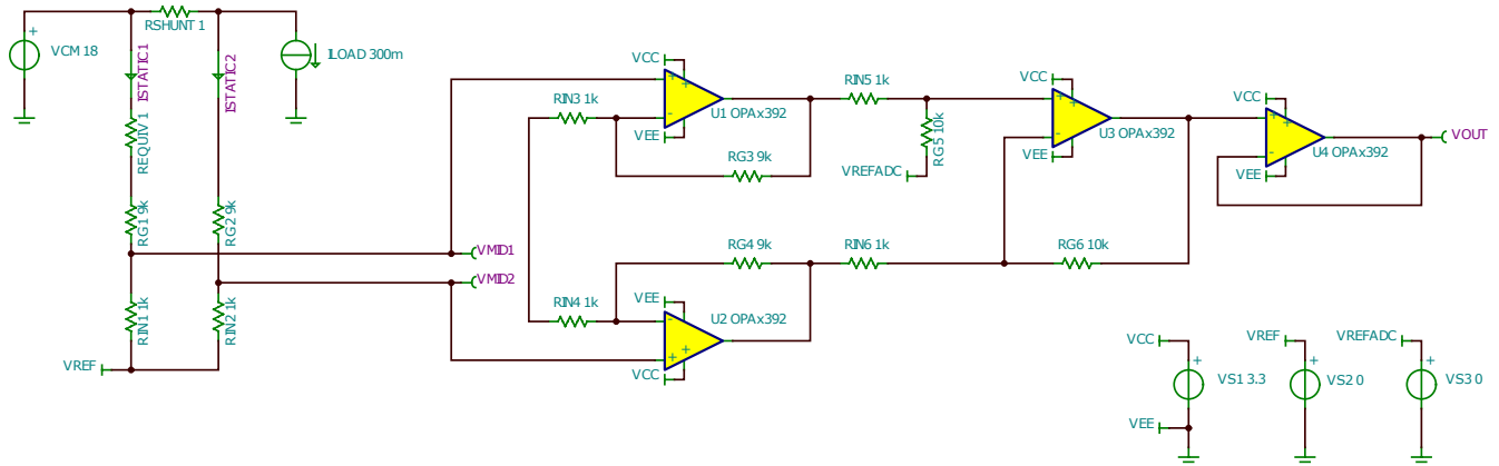
8-8. Circuit Model in TINA-TI
