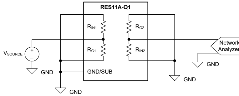
6-7. Crosstalk Measurement Reference Schematic
