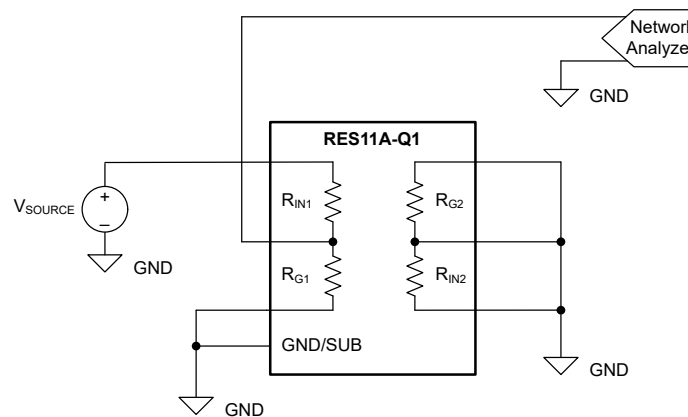
图 6-6. Bandwidth Measurement Reference Schematic
