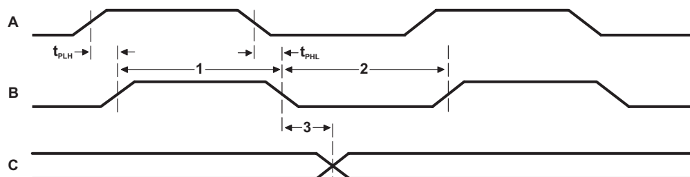
Figure 4-67. Trace Timing
