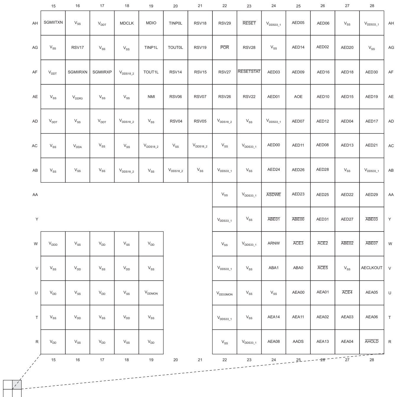
Figure 3-3. TCI648F Pin Map (Bottom View) [Quadrant B]
