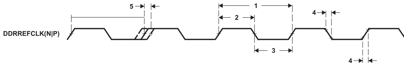
Figure 4-30. DDRREFCLK(N|P) Timing
