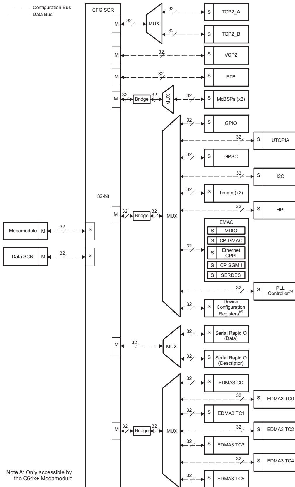
Figure 5-10. Configuration Switched Central Resource (SCR) Block Diagram
