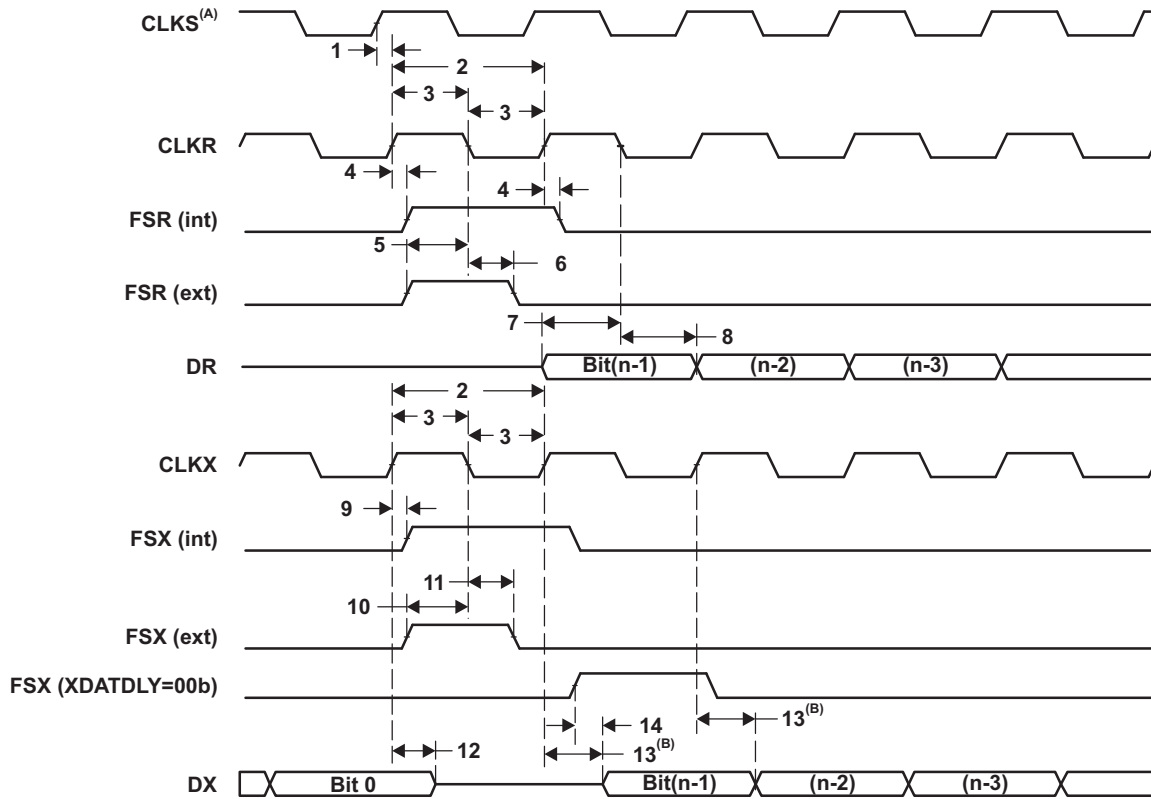
Figure 4-51. McBSP Timing
