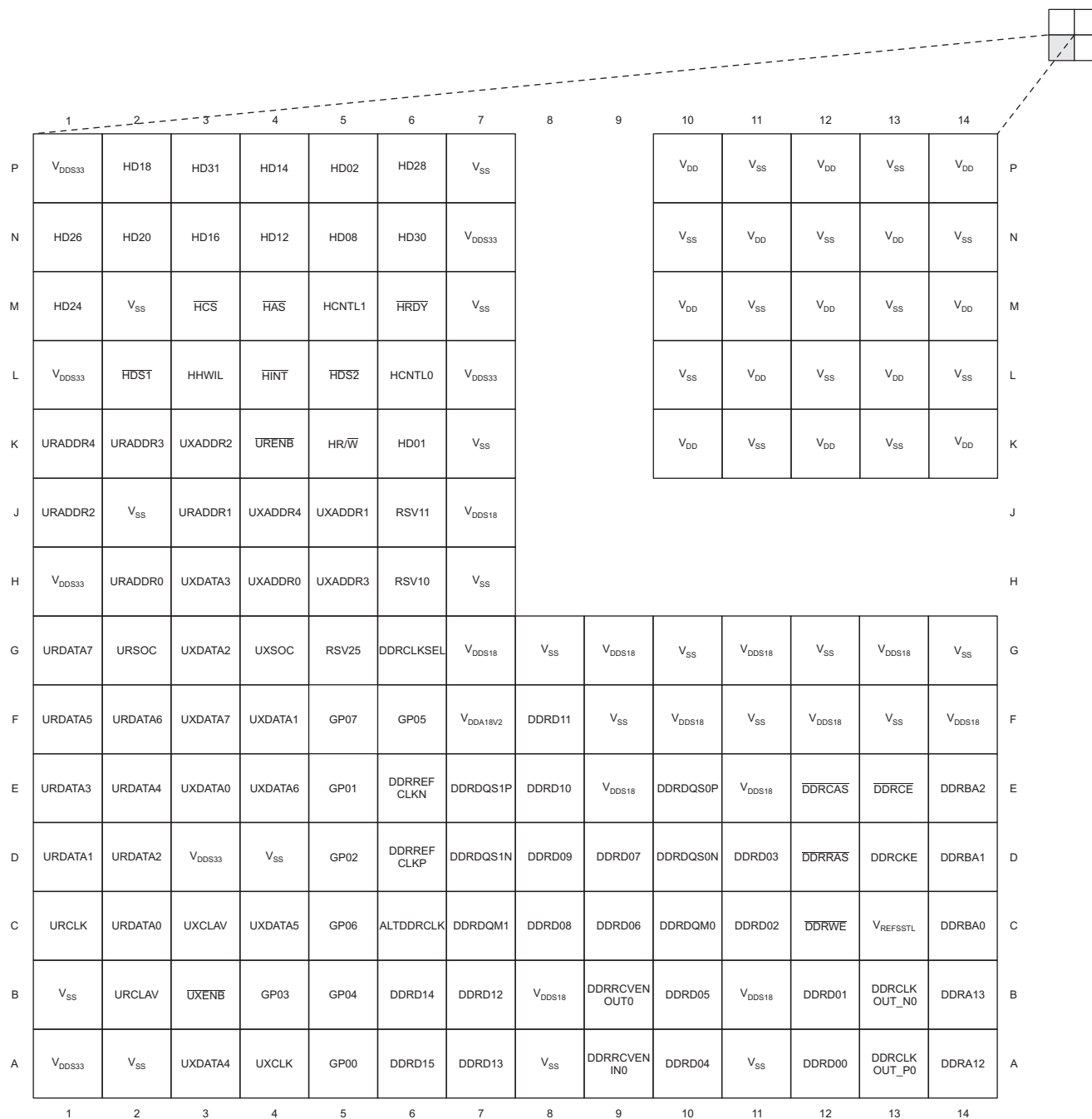
Figure 3-5. TC1648F Pin Map (Bottom View) [Quadrant D]
