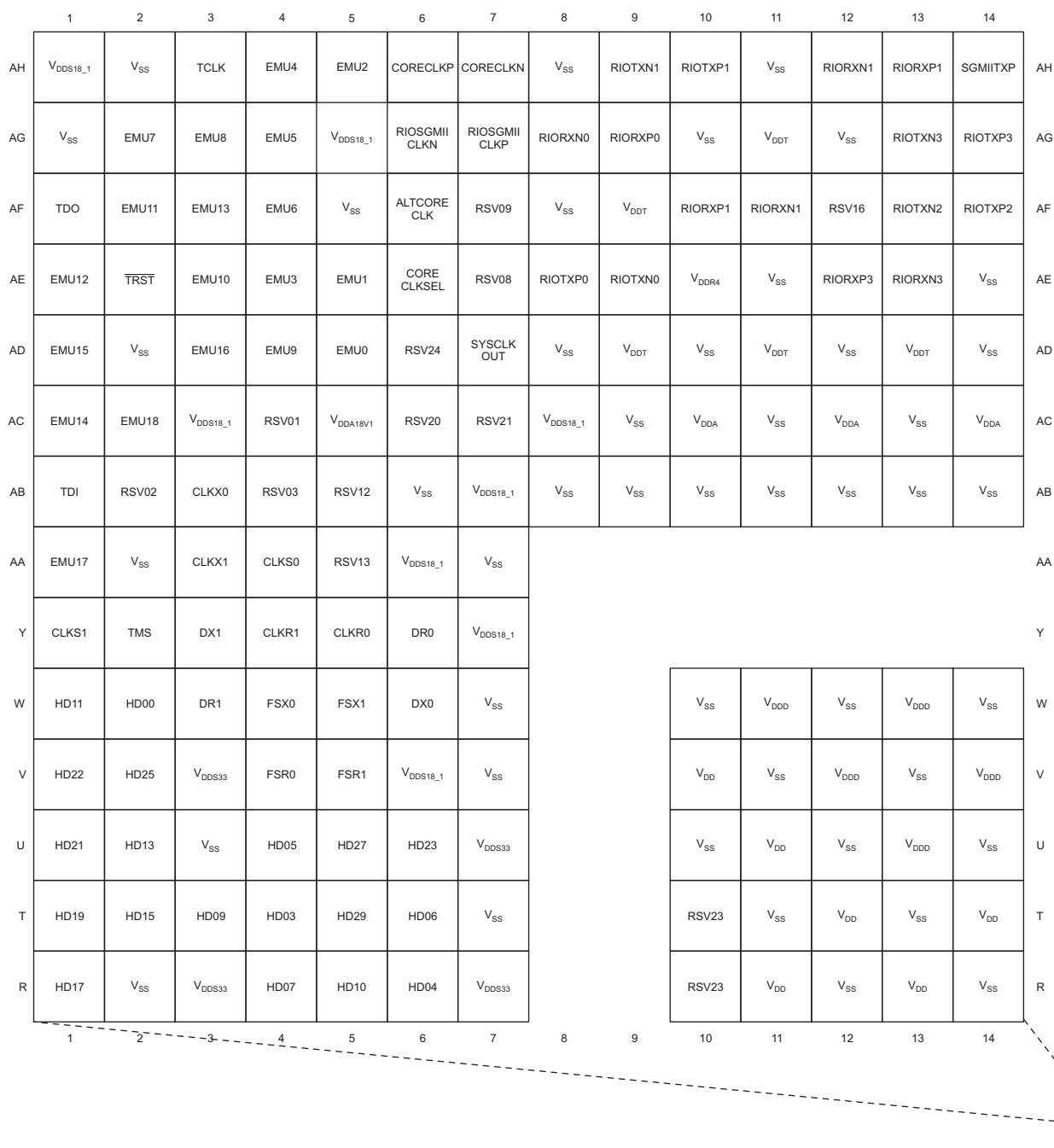
Figure 3-2. SM320C6457-HIREL Pin Map (Bottom View) [Quadrant A]
