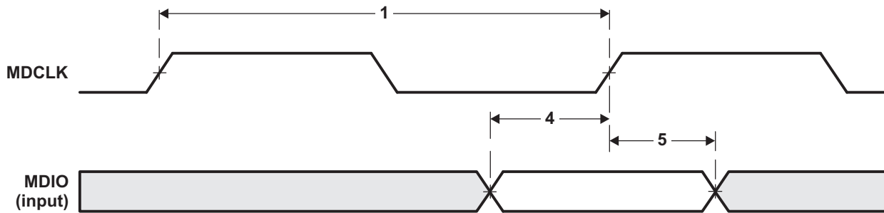
Figure 4-58. MDIO Input Timing
