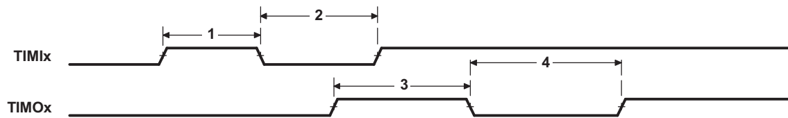
Figure 4-61. Timer Timing
