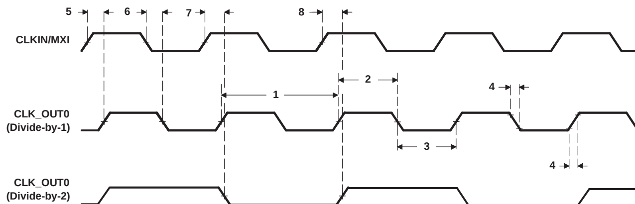
Figure 6-16. CLK_OUT0 Timing
