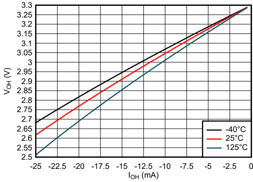
图 5-7. Output Voltage vs Current in HIGH State; 3.3-V Supply
