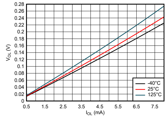
图 5-12. Output Voltage vs Current in LOW State; 1.8-V Supply
