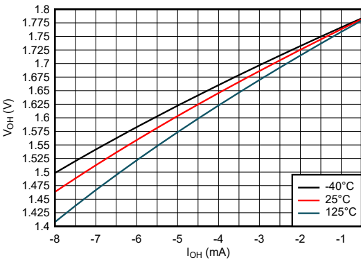
图 5-11. Output Voltage vs Current in HIGH State; 1.8-V Supply
