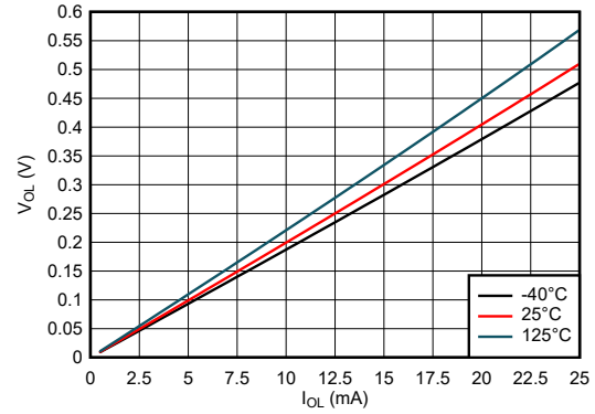
图 5-8. Output Voltage vs Current in LOW State; 3.3-V Supply
