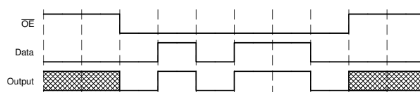
8-2. Application Timing Diagram
