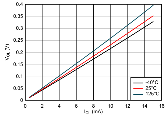
图 5-10. Output Voltage vs Current in LOW State; 2.5-V Supply
