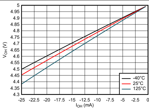
5-5. Output Voltage vs Current in HIGH State; 5-V Supply
