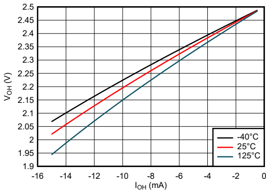
图 5-9. Output Voltage vs Current in HIGH State; 2.5-V Supply
