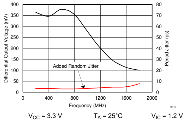
6-12. Differential Output Voltage vs Frequency
