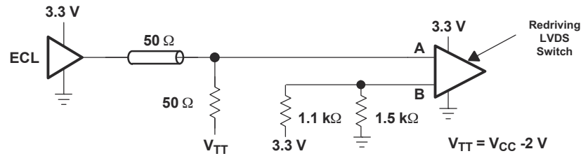
図 9-3. Single-Ended (LVPECL)
