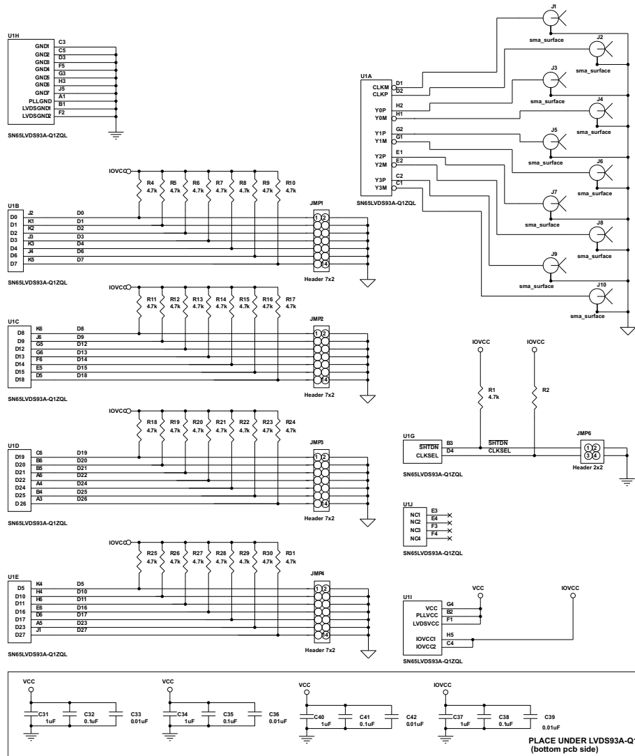
14. Schematic Example (SN65LVDS93A Evaluation Board)
