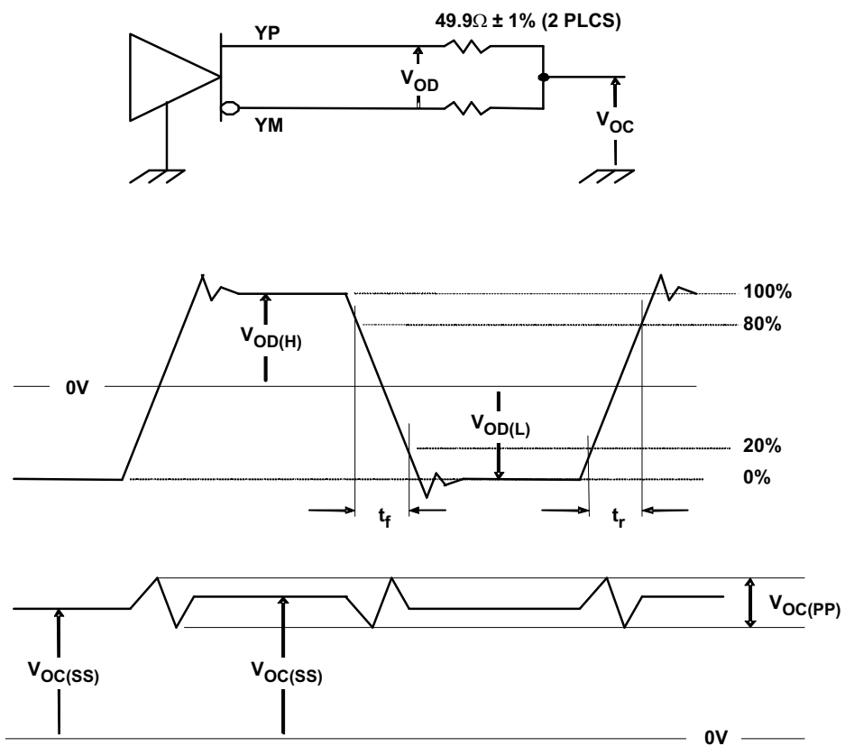
Fig. 7. Test Load and Voltage Definitions for LVDS Outputs
