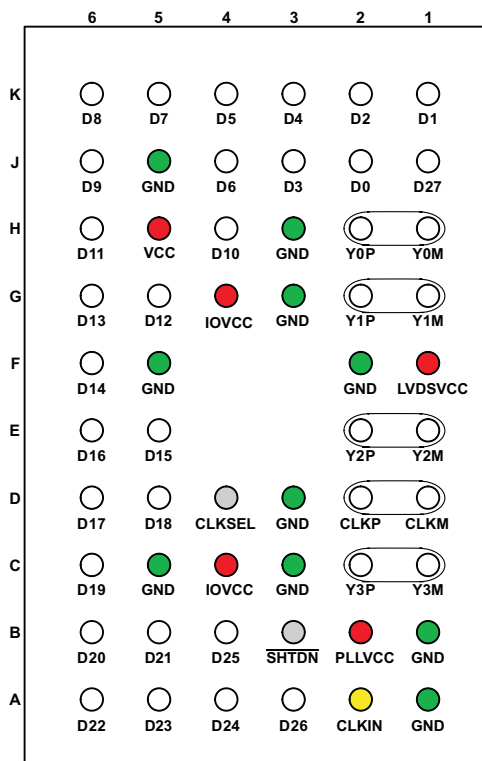
ZQL Package 56-Ball BGA MICROSTAR (Top View)
