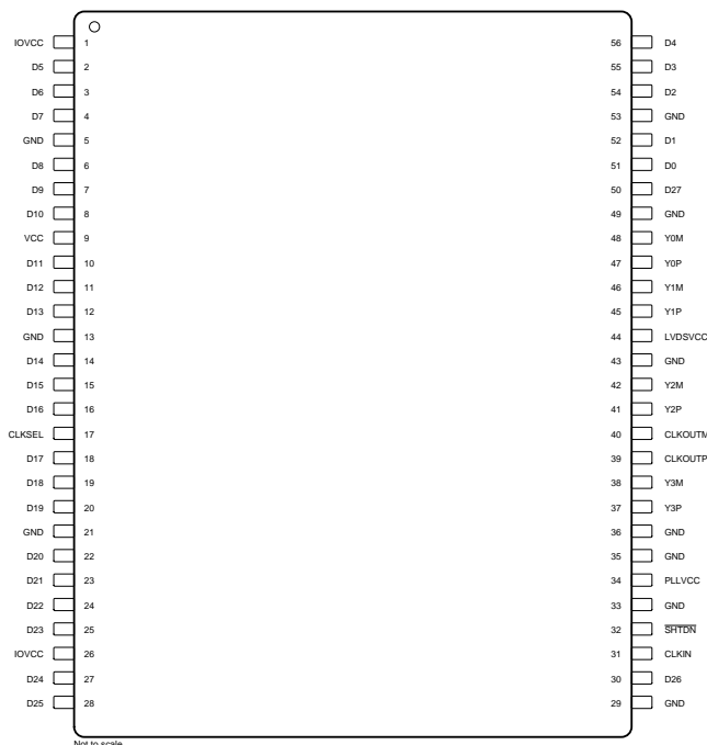
DGG Package 56-Pin TSSOP (Top View)
