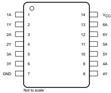
図 4-1. D, DB, DGV, J, N, NS, PW, or W Package, 14-Pin SOIC, SSOP, TVSOP, CDIP, PDIP, SO, TSSOP, or CFP (Top View)
