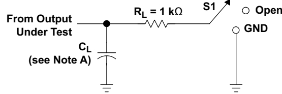
LOAD CIRCUIT FOR 3-STATE AND OPEN-DRAIN OUTPUTS
