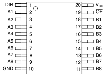
図 5-1. SN54AHCT245: J or W SN74AHCT245: DB, DGV, DW, N, NS, PW or DGS Package, 20-Pin CDIP, CFP, SSOP, TVSOP, SOIC, PDIP, SOP, TSSOP, or VSSOP (Top View)
