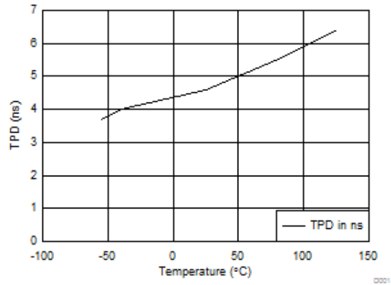
FIG 6-1. SNx4AHCT245 TPD vs Temperature, 15 pF Load
