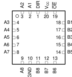
図 5-3. SN54AHCT245: FK Package, 20-Pin LCCC (Top View)
