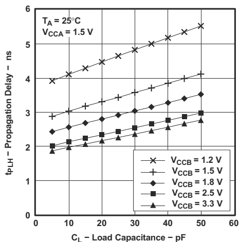
6-3. Typical Propagation Delay t_{PLH} (A to B) vs Load Capacitance
