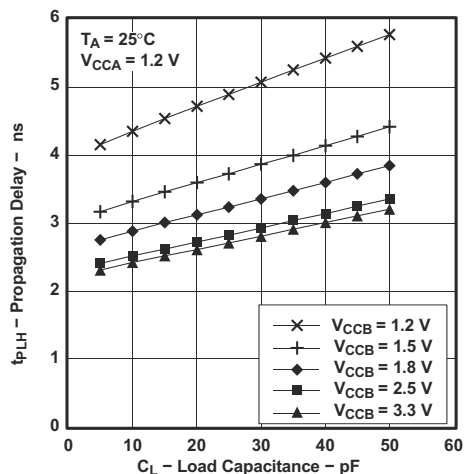
6-1. Propagation Delay vs Load Capacitance
