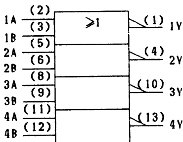
LOGIC SYMBOL
