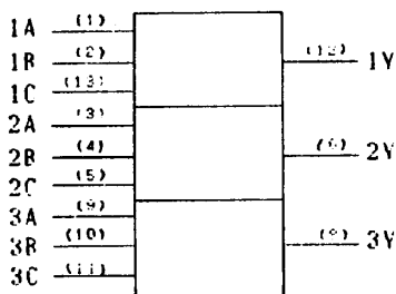
LOGIC SYMBOL
