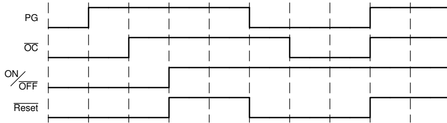
⊠ 10. Application timing diagram
