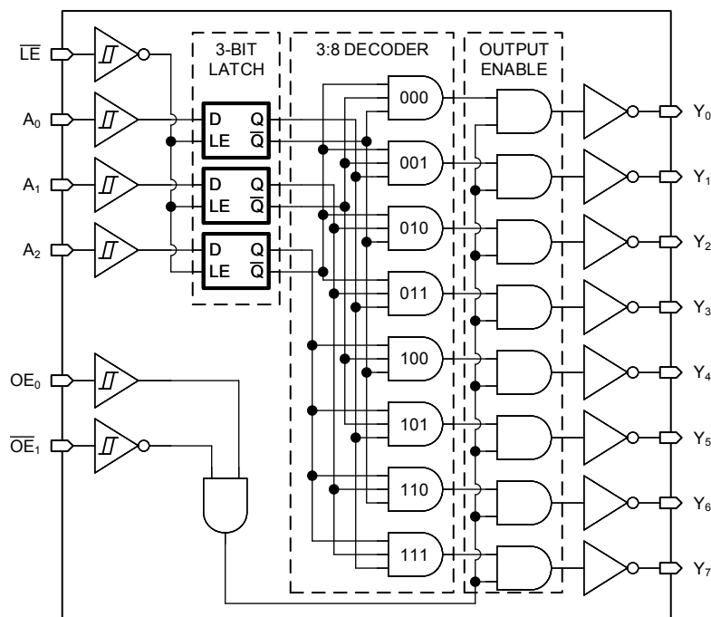
FIG 8-1. Logic Diagram (Positive Logic) for the SN74HCS137
