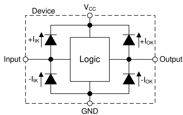
FIG 8-2. Electrical Placement of Clamping Diodes for Each Input and Output
