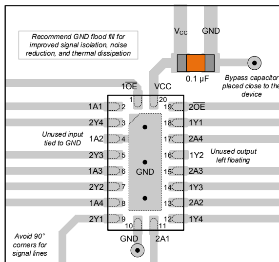
11-2. Example Layout for the SN74HCS244 in the RKS Package
