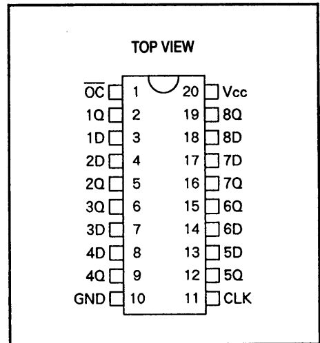
PIN ASSIGNMENT
