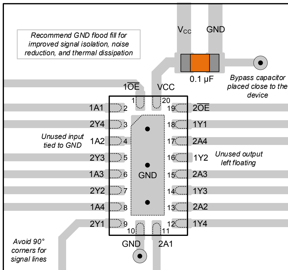
✎ 9-3. Layout Example for the SN74LV244A-Q1 in the WRKS Package
