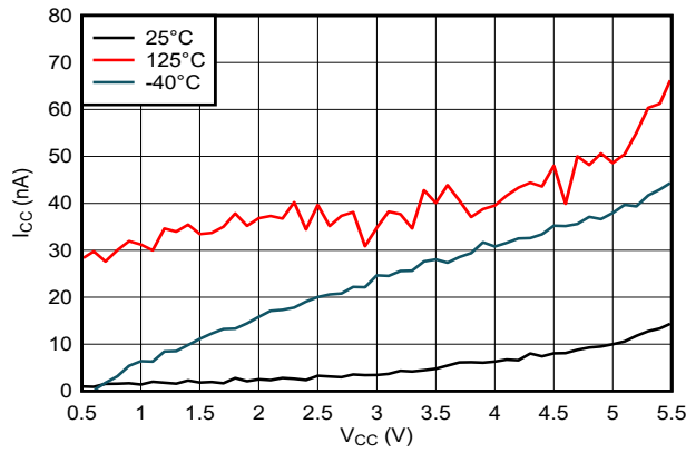
図 5-3. Supply Current Across Supply Voltage
