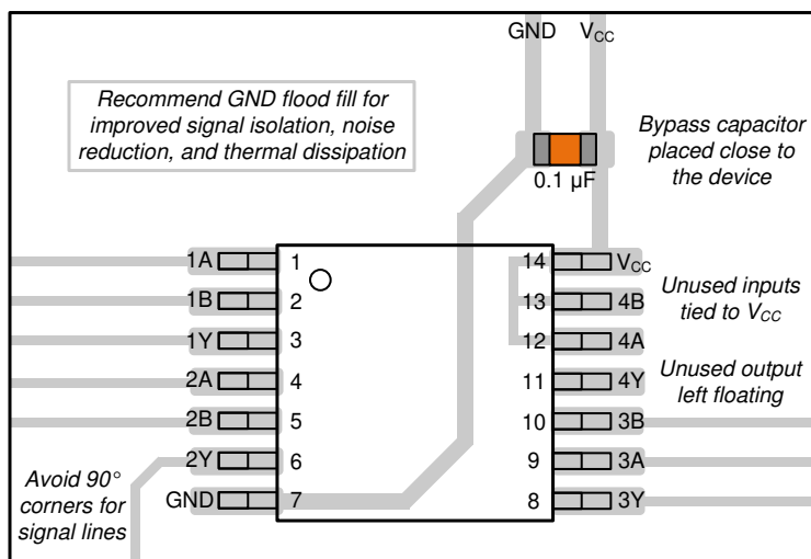
FIG 12-1. Example Layout for the SN74LV4T08-Q1
