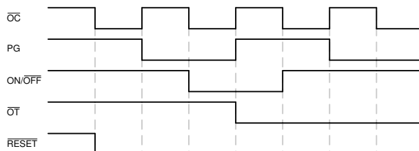
FIG 10-2. Application Timing Diagram
