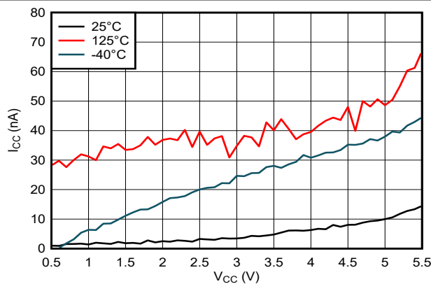
FIG 6-3. Supply Current Across Supply Voltage
