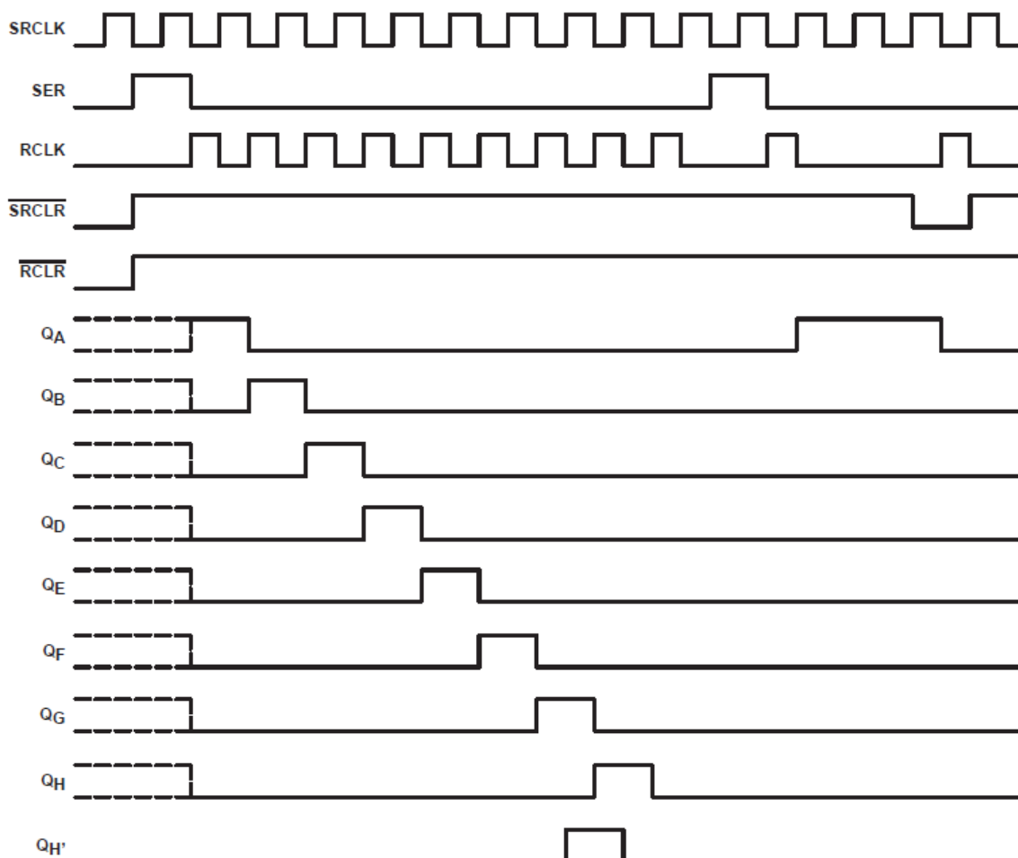
6-1. Timing Diagram
