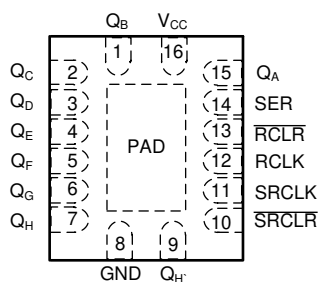
图 5-1. D, DB, or PW Package 16-Pin SOIC, SSOP, or TSSOP (Top View)
