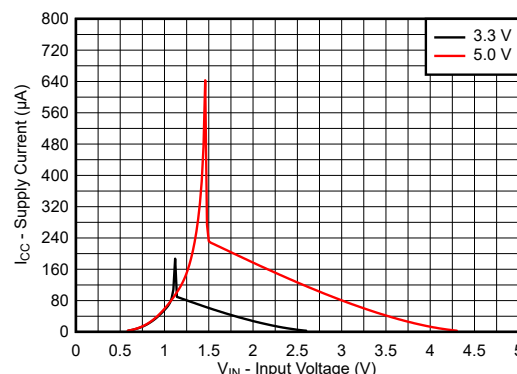
6-2. Supply Current Across Input Voltage 3.3-V and 5.0-V Supply
