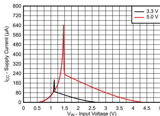
FIG 7-2. Supply Current Across Input Voltage 3.3-V and 5.0-V Supply
