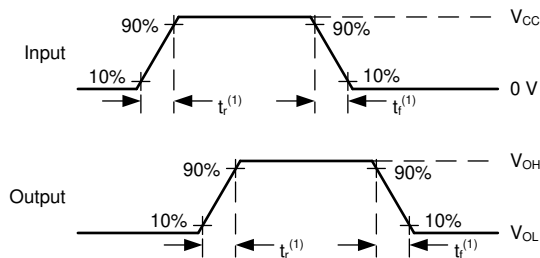
FIG 8-3. Voltage Waveforms, Input and Output Transition Times
