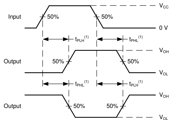
FIG 8-2. Voltage Waveforms Propagation Delays
