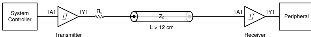
图 10-1. Typical Application Block Diagram
